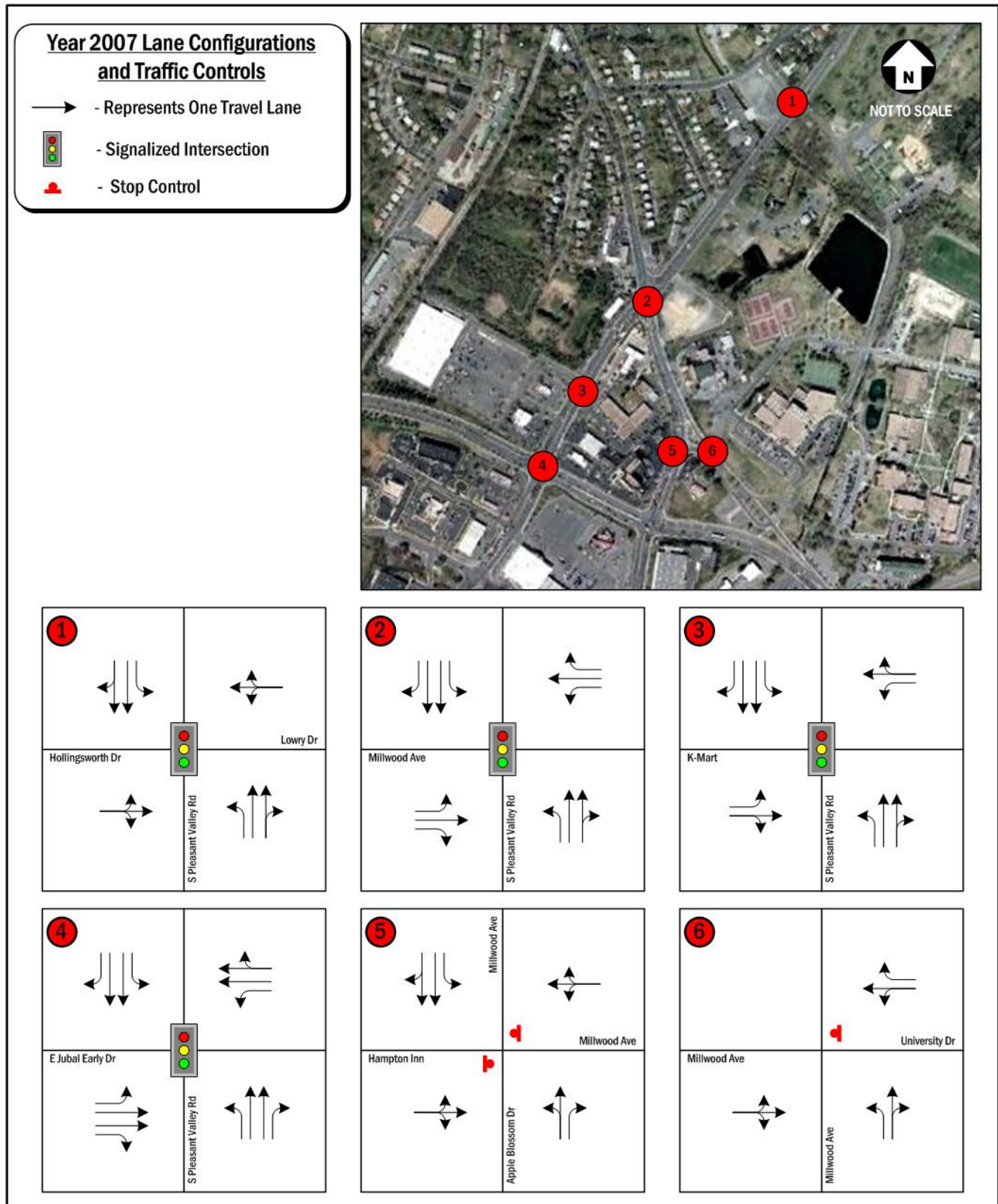
Figure 27: Year 2007 Lane Configurations and Traffic Controls (1 of 2)
