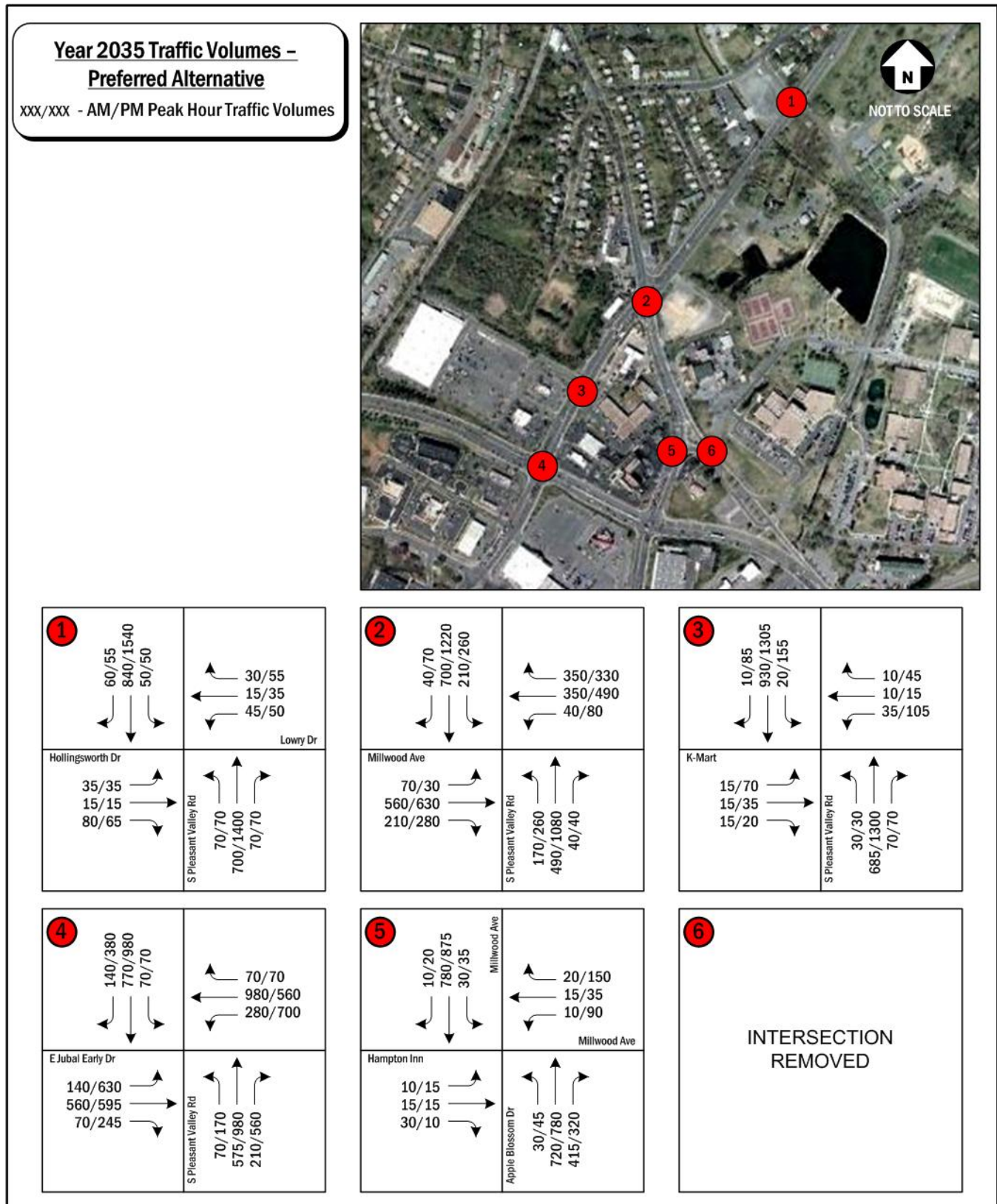
Figure 25: Year 2035 Conditions Traffic Volumes, Preferred Alternative (1 of 2)
