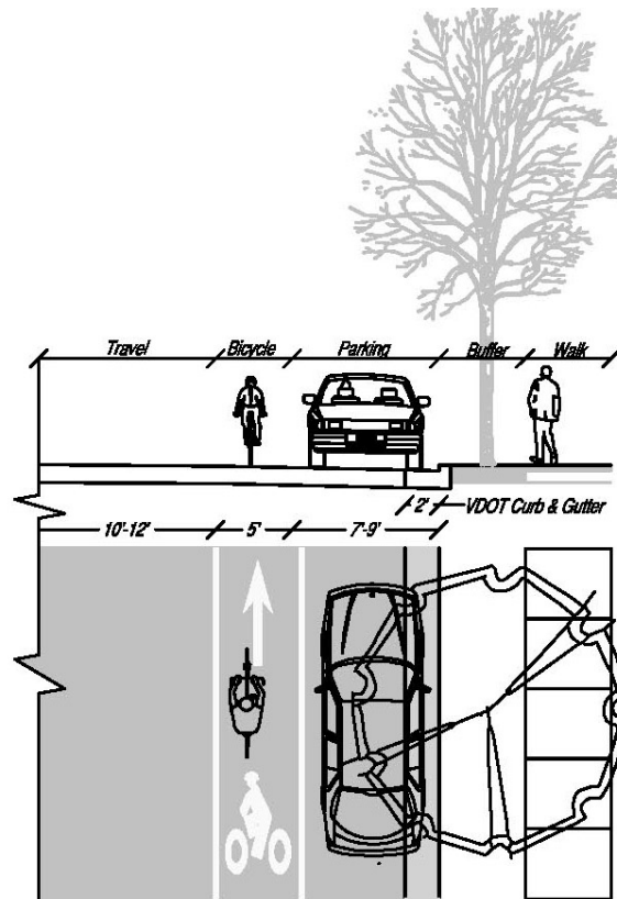
Bicycle lane on roadway with parking, ≤ 30 mph
