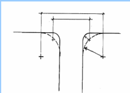
Figure 8. Plan-view diagram of a street intersection. Reducing the radius of street corners slows turning vehicle traffic and shortens pedestrian crosswalks.
