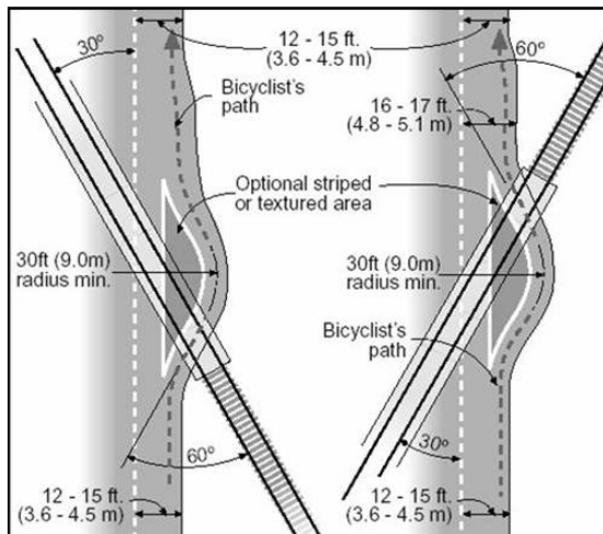
Skewed Railroad Crossing in Madison, Wisconsin
