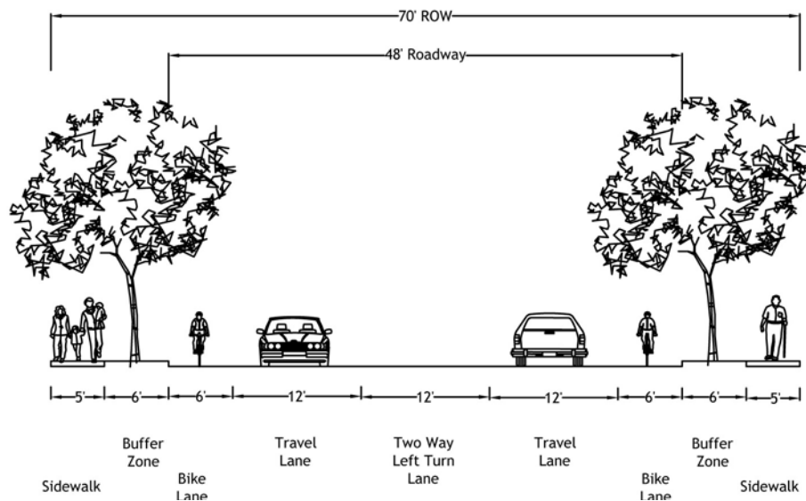
City of Winchester Category III Street: Shown with 2 lanes with two-way left turn lane, bike lanes, buffer zones, and sidewalks (widen sidewalks if in a commercial area)
